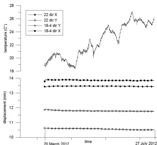
Fig. 16: Time- displacement-temperature curves for two cracks (in X and Y directions).
