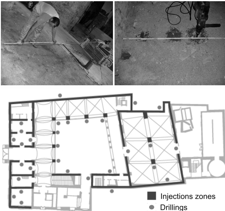
Fig. 2: Above: foundation survey at Palatium Vetus. Below: survey and intervention map.
