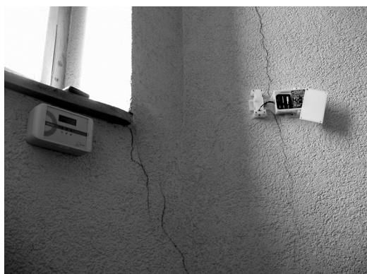
Fig. 15: Easy Crack Monitor System®.
